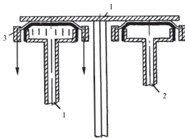
48-rasm. TI-1M asbobining shakli: 1 — disk; 2 — boshchasi; 3 — namuna.
